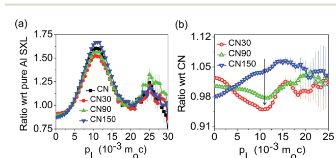
Fig. 5 (a) Ratio curves of the area-normalized CDB spectra of pure and plasma-treated samples with respect to 99.9999% pure Al. (b) CDB spectra of plasma-treated samples with respect to pure CN.
