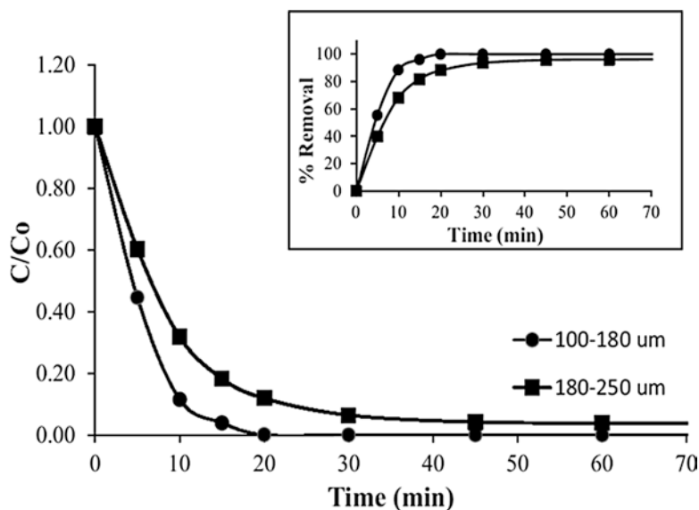
Fig. 16.4 Effect of Poly[(2-methacryloyloxy)ethyl]trimethylammonium chloride) chelating resin particle size on chromium(VI) removal percentage. A 95% chromium(VI) removal was reached using particle sizes from 100 to 180 \mu\text{m} , meanwhile with particle sizes from 180 to 250 \mu\text{m} this percentage is obtained after 45 min only. (Reprinted with permission of the copyright holders, Springer from Santander et al. 2017)
