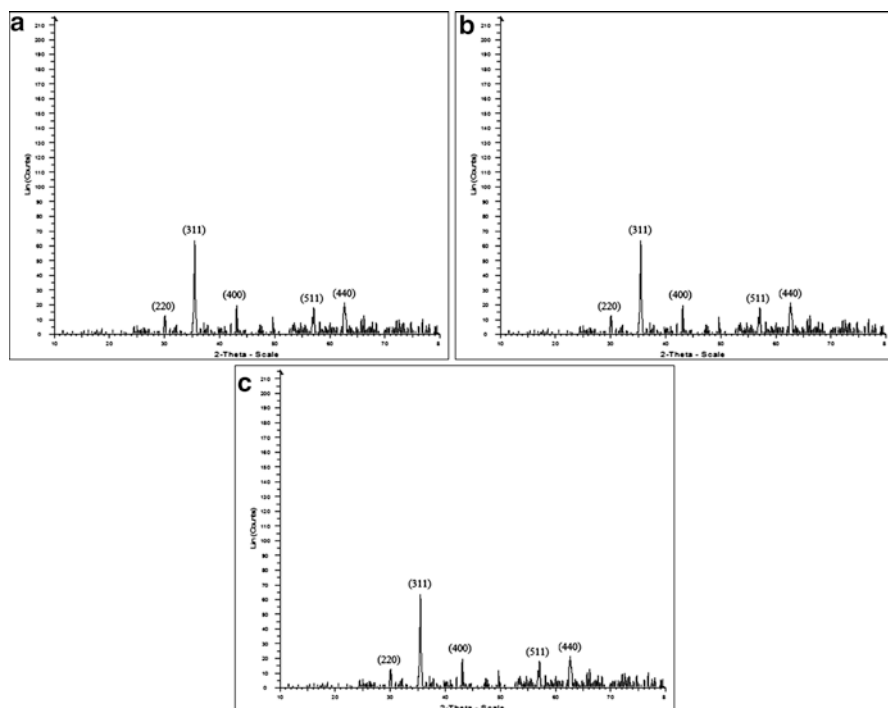
Fig. 3.6 XRD diffractogram of (a) \text{Fe}_2\text{O}_3 @EFB (Daneshfozoun et al. 2017), (b) \text{Fe}_2\text{O}_3 @CEL, (c) \text{Fe}_2\text{O}_3 @RKF. The results show distinctive peak at 2\theta = 30.1^\circ, 57.0^\circ, 35.5^\circ, 62.6^\circ and 43.1^\circ corresponding to (2 2 0), (5 1 1), (3 1 1), (4 4 0), (5 1 1) and (4 0 0) lattice properties. These are linked to the oxide of iron nanoparticles (PCPDFWIN v.2.02, PDF No. 85–1436). Point indicating deflection constituents in mass does not cause change in \text{Fe}_2\text{O}_3 nanoparticles. Similarly indicated are the XRD for Raw Kapok Fibers and cellulose composite
