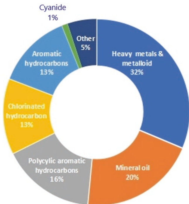
Fig. 8.1 Composition of water contaminants in recycled water. In recycled water 32% comprised of heavy metals and metalloids, 20% of mineral oil, 16% of polycyclic aromatic hydrocarbons, 13% of chlorinated hydrocarbon, 13% of aromatic hydrocarbon, 1% of cyanide, and 5% of other contaminants. (Modified from Bolisetty et al. 2019)
