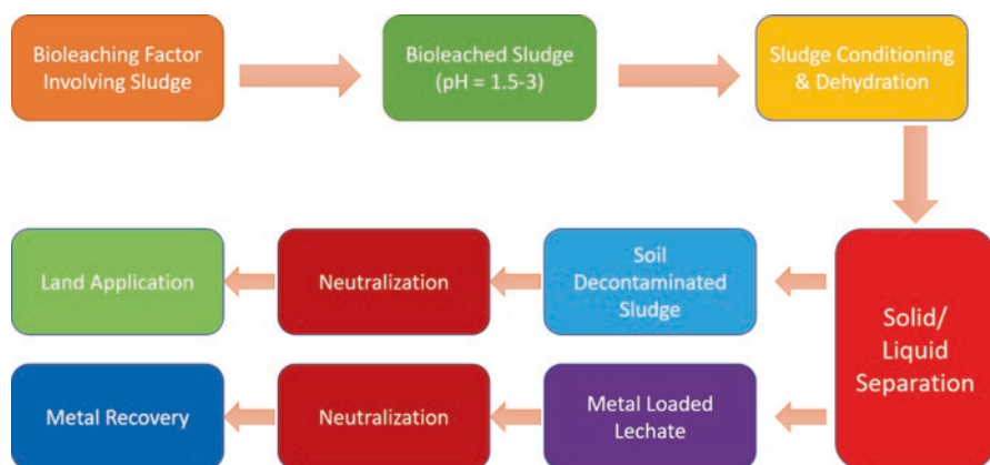
Fig. 8.13 Process of bioleaching. Bioleached sludge is conditioned and dehydrated leading to solid and liquid separation, thereby neutralizing it to obtain metal recovery. (Reprinted with permission of Bioleaching of heavy metals from sewage sludge: A review, Attribution international (CC BY 3.0), Pathak et al. 2009)
