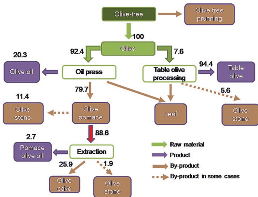
Fig. 2.1 Diagram of the olive processing. (Adapted to AGAPA 2015)
