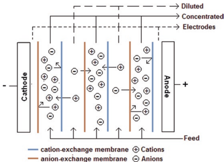
Fig. 5.1 Electrodialysis principle. Cations and anions from a feed solution are selectively transferred through alternated cation- and anion-exchange membranes producing diluted and concentrated solutions. Modified after Marder et al. (2003)
