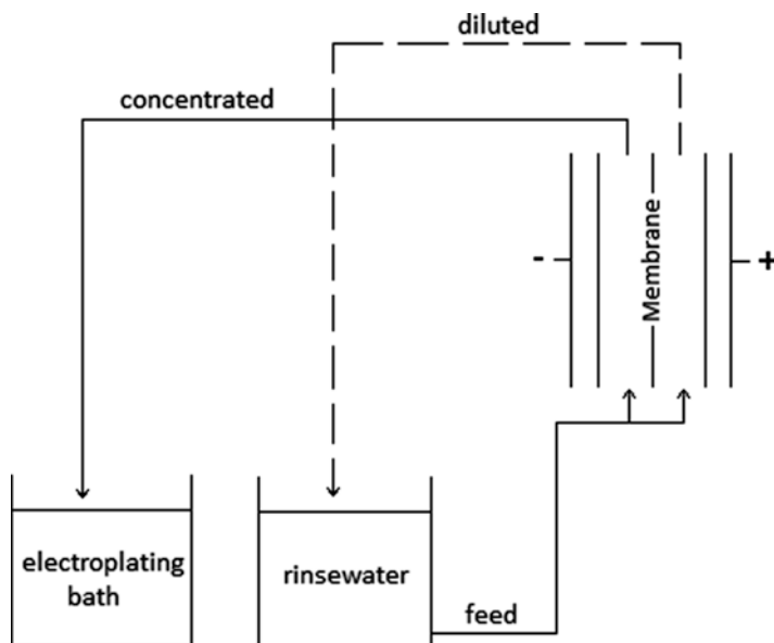
Fig. 5.2 Flow chart illustrating the application of electrodialysis in the galvanic process. Exhausted rinsewater is diluted and concentrated by an electrodialyzer allowing the recovery of chemicals and water in the process. Modified after Chiapello and Gal (1992)
