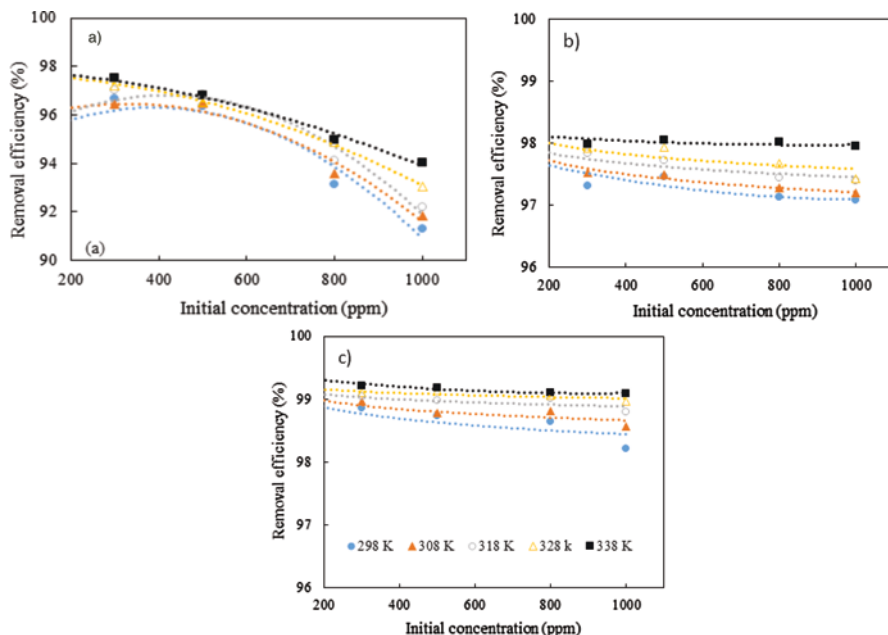
Fig. 3.9 Effects of temperature and concentration on the removal of lead showing that the differently modified sorbents had different effects on the heavy metals (a) \text{Fe}_2\text{O}_3@\text{EFB} , (b) \text{Fe}_2\text{O}_3@\text{CEL} , (c) \text{Fe}_2\text{O}_3@\text{RKF} (Reprinted with the permission from [Preparation and characterization of magnetic biosorbent based on oil palm empty fruit bunch fibers, cellulose and Ceiba pentandra for heavy metal ions removal, Daneshfozoun et al. 2017, Elsevier])
