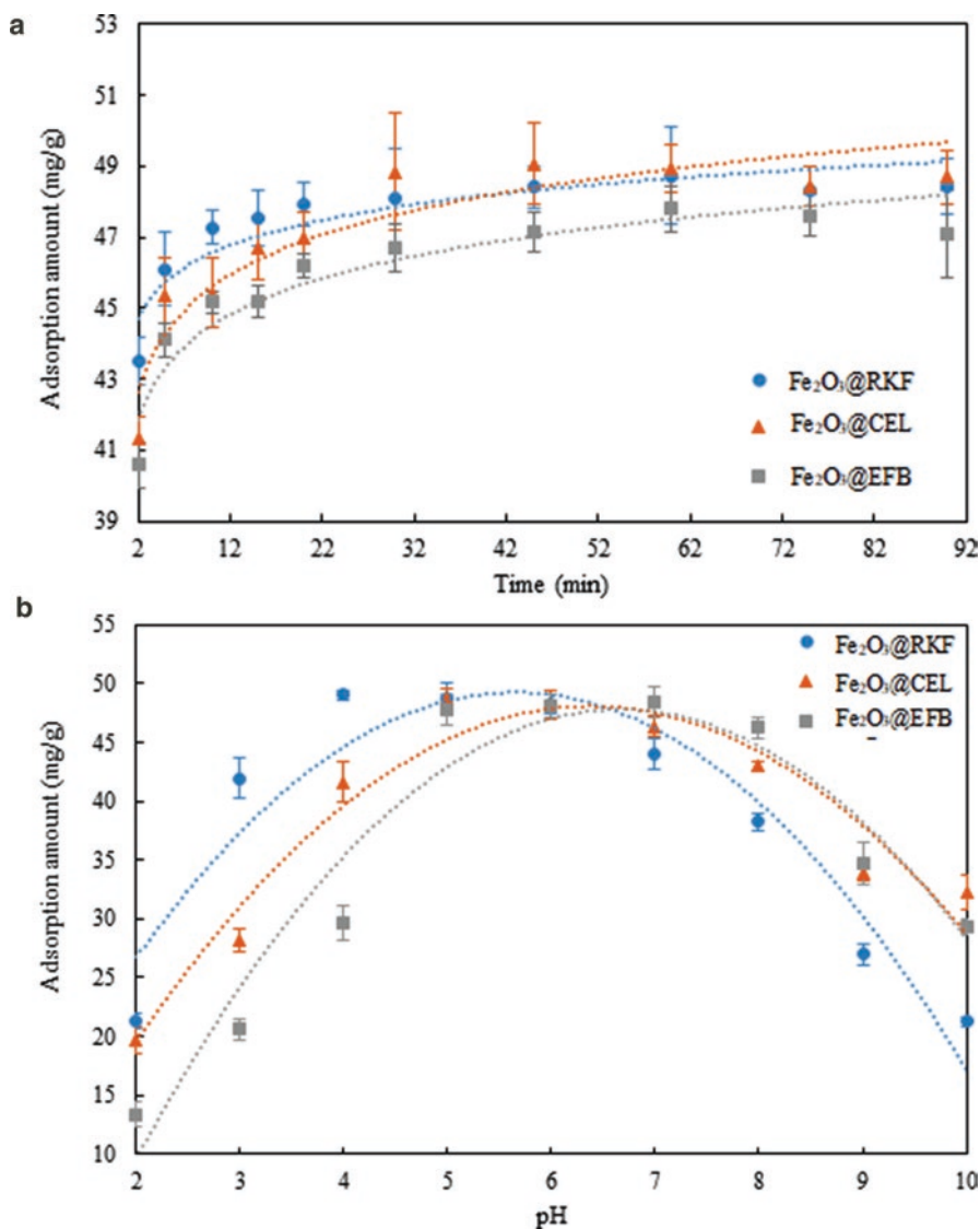
Fig. 3.8 Influence of (a) contact time on impurities sorption by differently altered magnetite, (b) solution pH, on lead adsorption by modified \text{Fe}_2\text{O}_3 . (Reprinted with permission from [Preparation and characterization of magnetic biosorbent based on oil palm empty fruit bunch fibers, cellulose and Ceiba pentandra for heavy metal ions removal, Daneshfozoun et al. 2017, Elsevier])
