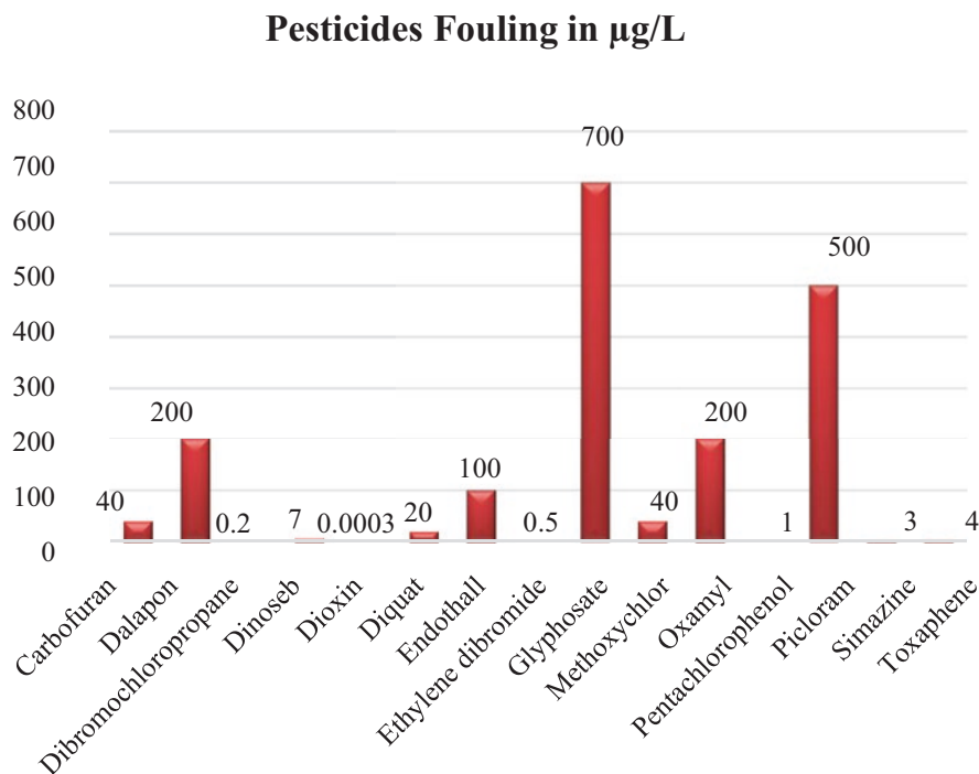
Fig. 13.4 This bar graph plotted between the different types of pesticides chemicals versus their fouling concentration in \mu\text{g/L} . Glyphosate is herbicide showed the maximum concentration to contaminant. (WHO 2009)
