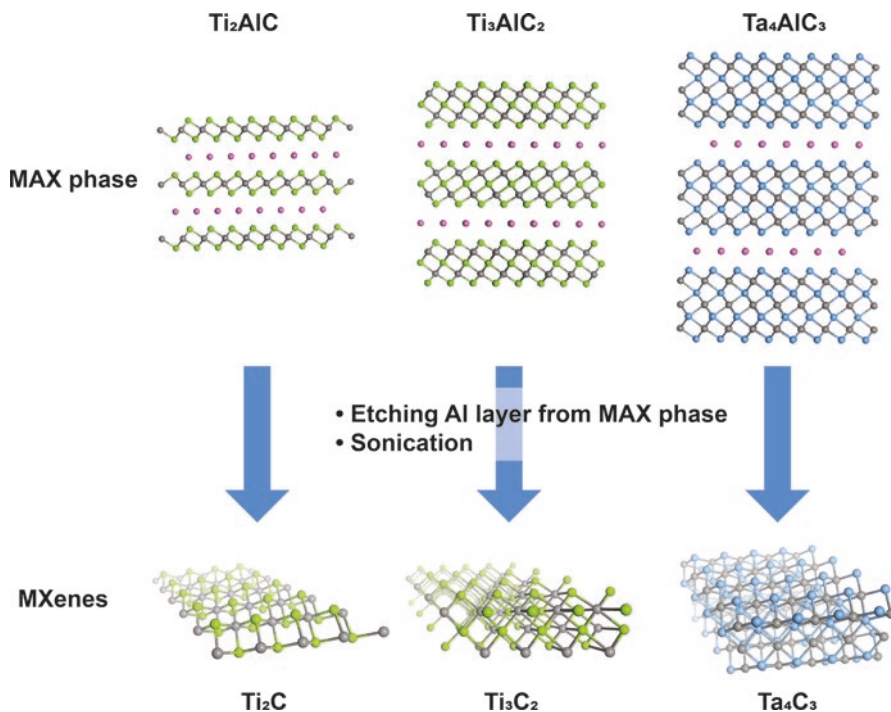
Fig. 4.5 Crystal structures of typical MAX phases ( \text{Ti}_2\text{AlC} , \text{Ti}_3\text{AlC}_2 , and \text{Ta}_4\text{AlC}_3 ) and the corresponding achieved MXenes through etching method ( \text{Ti}_2\text{C} , \text{Ti}_3\text{C}_2 , and \text{Ta}_4\text{C}_3 ). The color scheme: pink ball: aluminum; black ball: carbon atom; green ball: titanium atom; blue ball: tantalum atom
